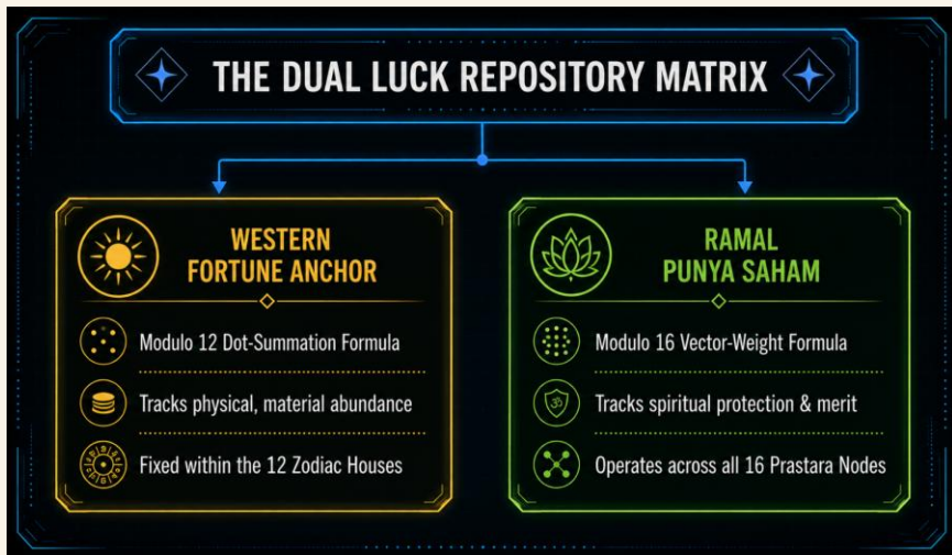
Figure 4.17.3: Punya Saham
